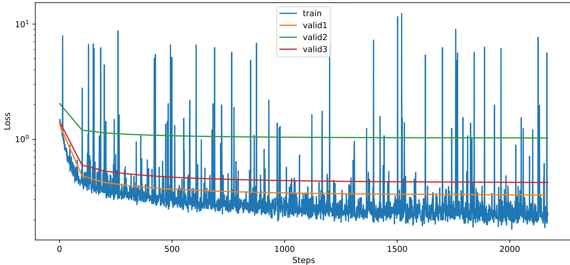
Training NMSE of TST_indiv
