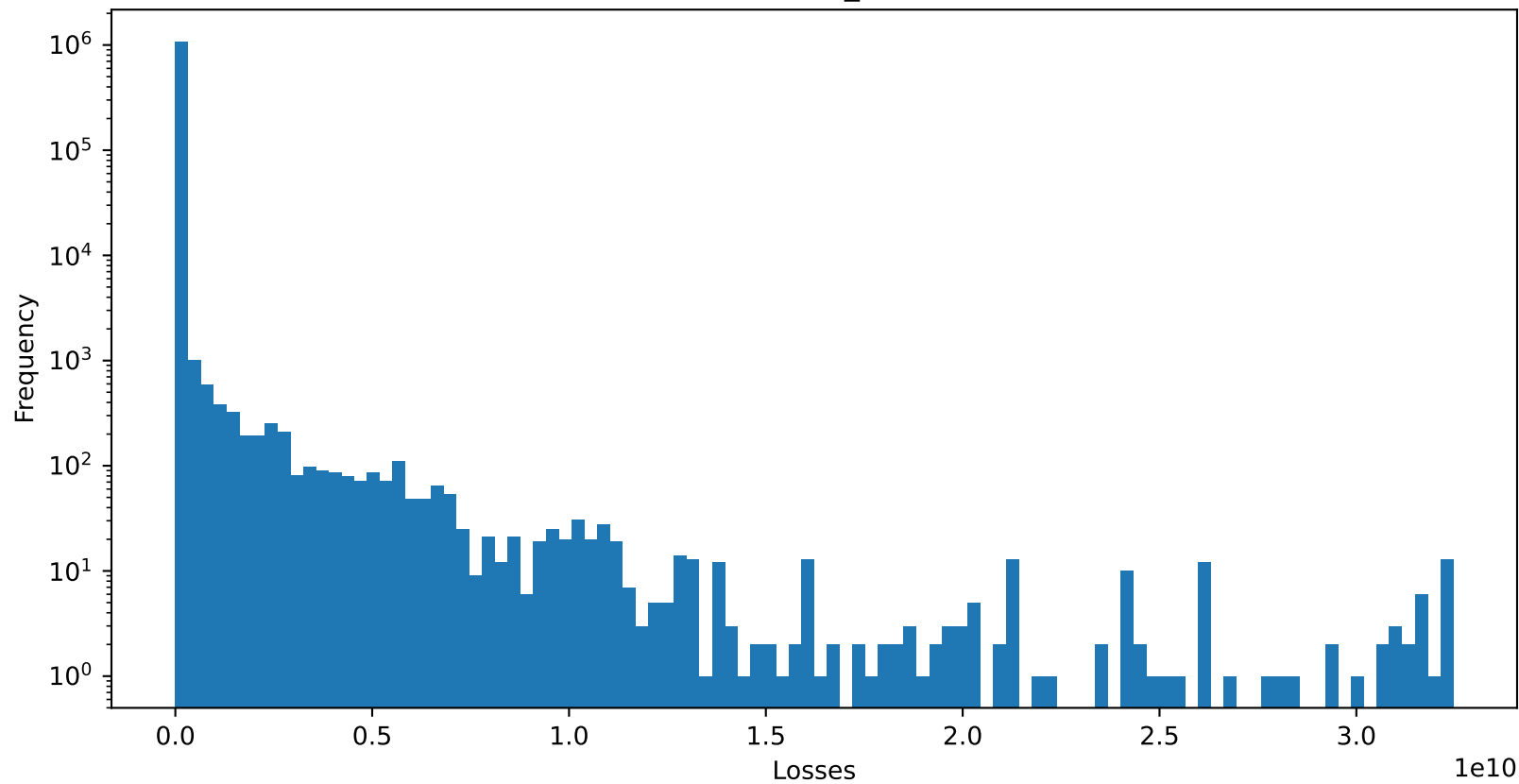
Test 1 MSE of lookback_168 : 14395180.0
