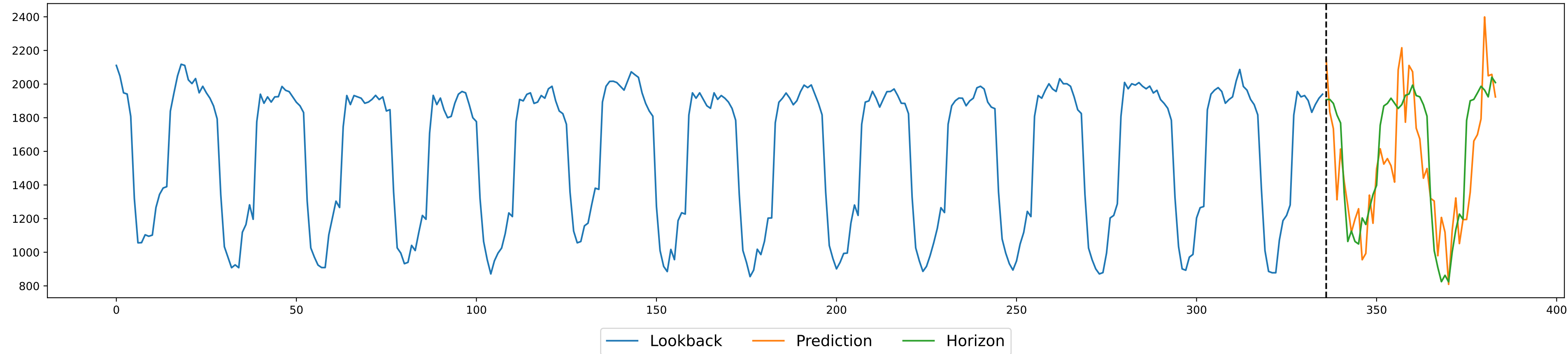
Example rand prediction for DLinear
