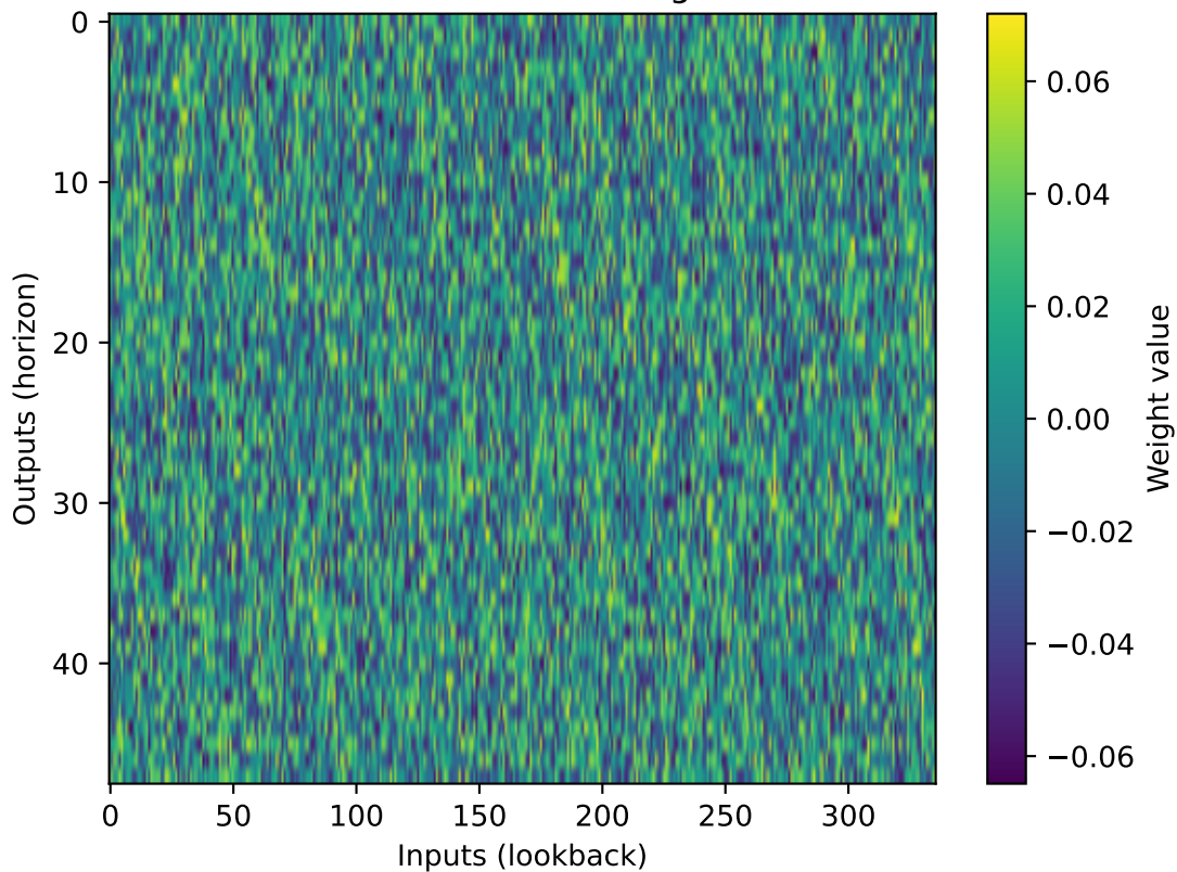
DLinear seasonal weights
