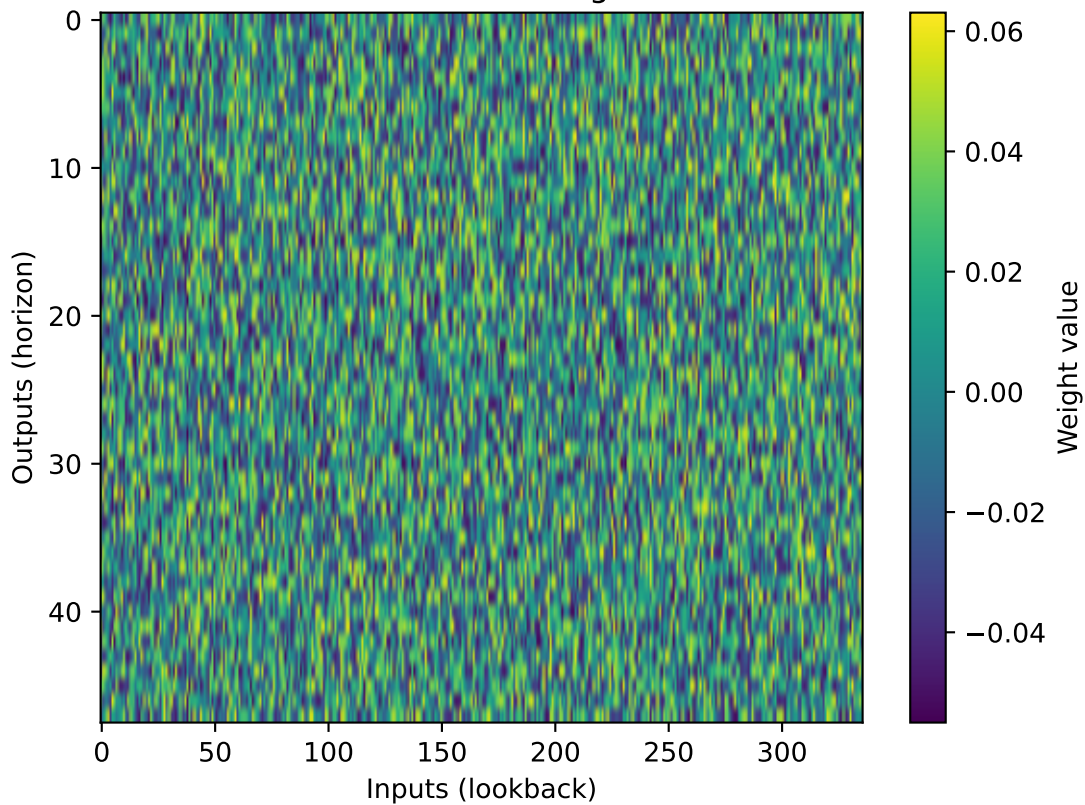
DLinear trend weights
