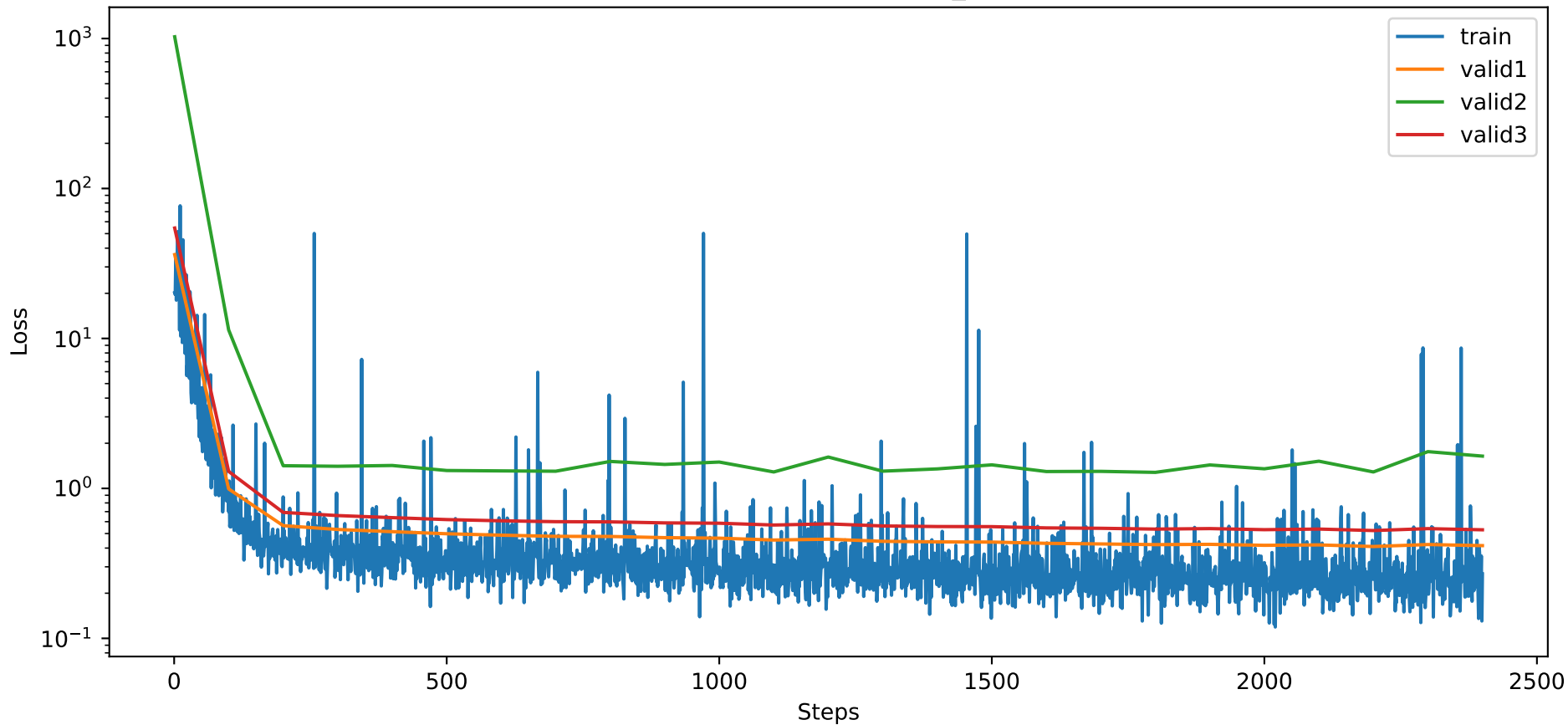
Training NMSE of DLinear_NMSE
