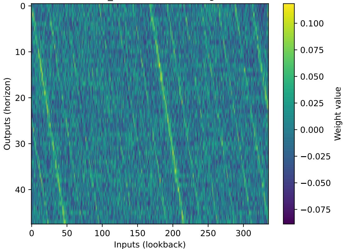
DLinear_NMSE seasonal weights
