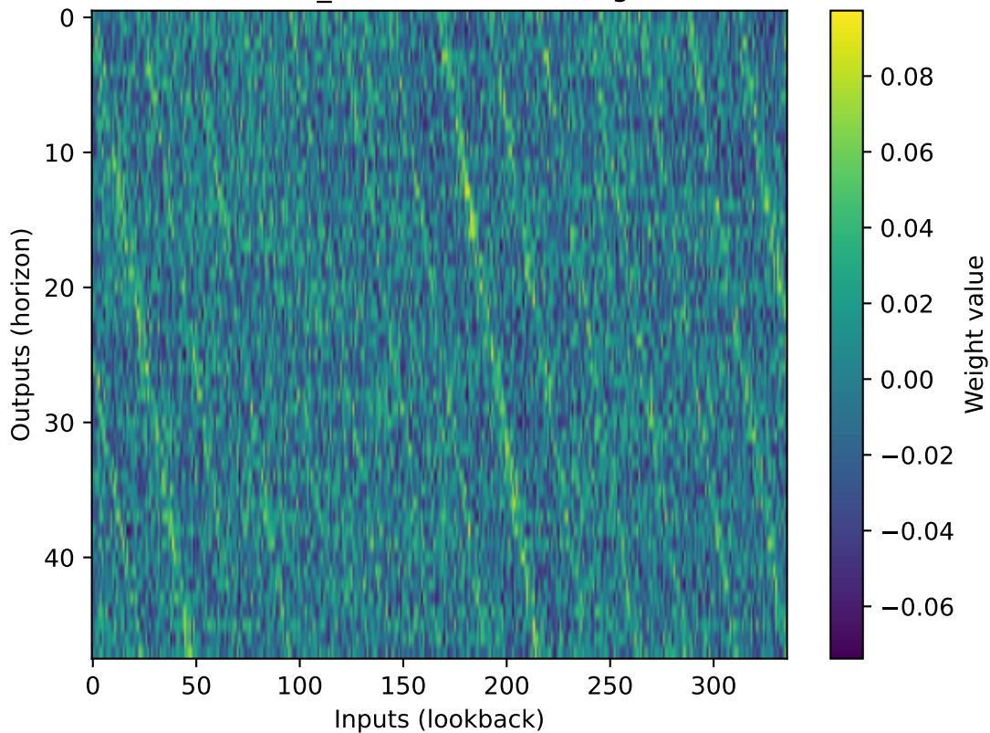
DLinear_RMSE seasonal weights
