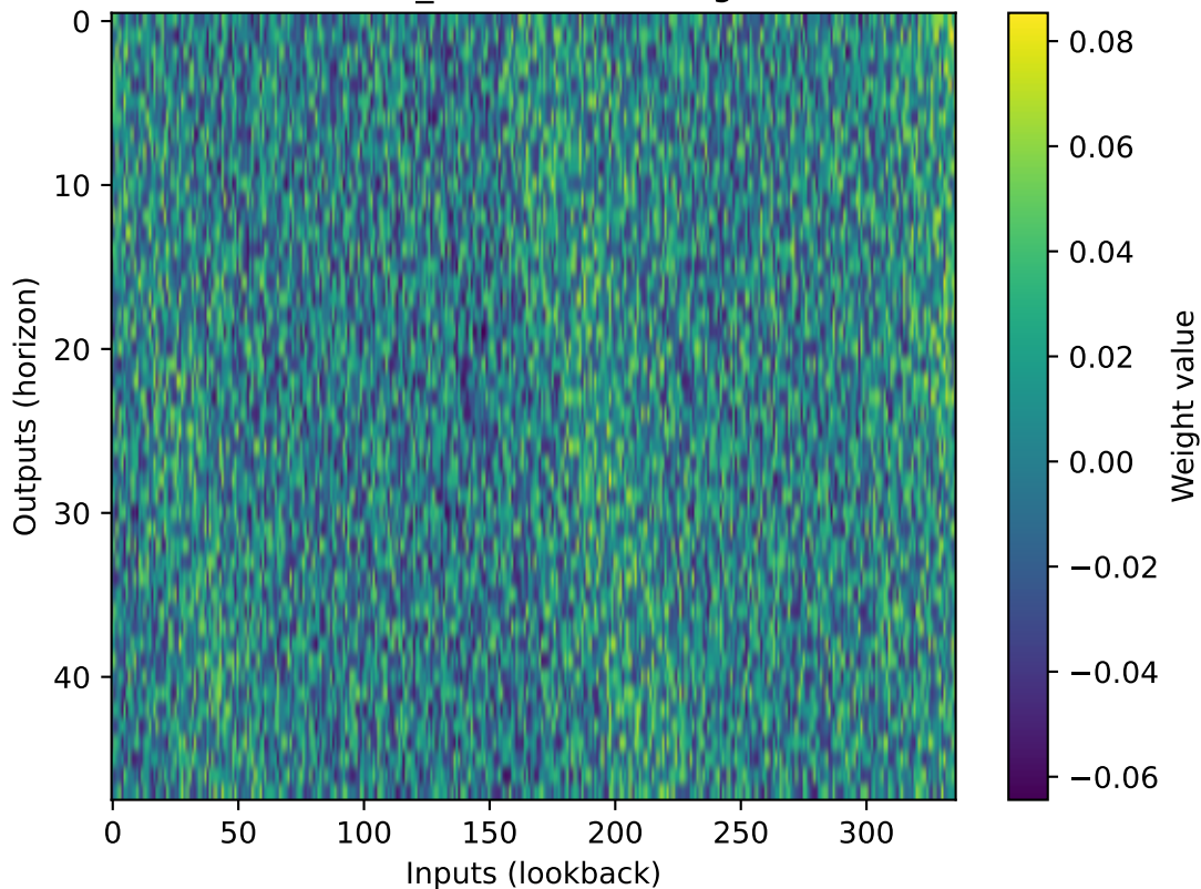
DLinear_RMSE trend weights
