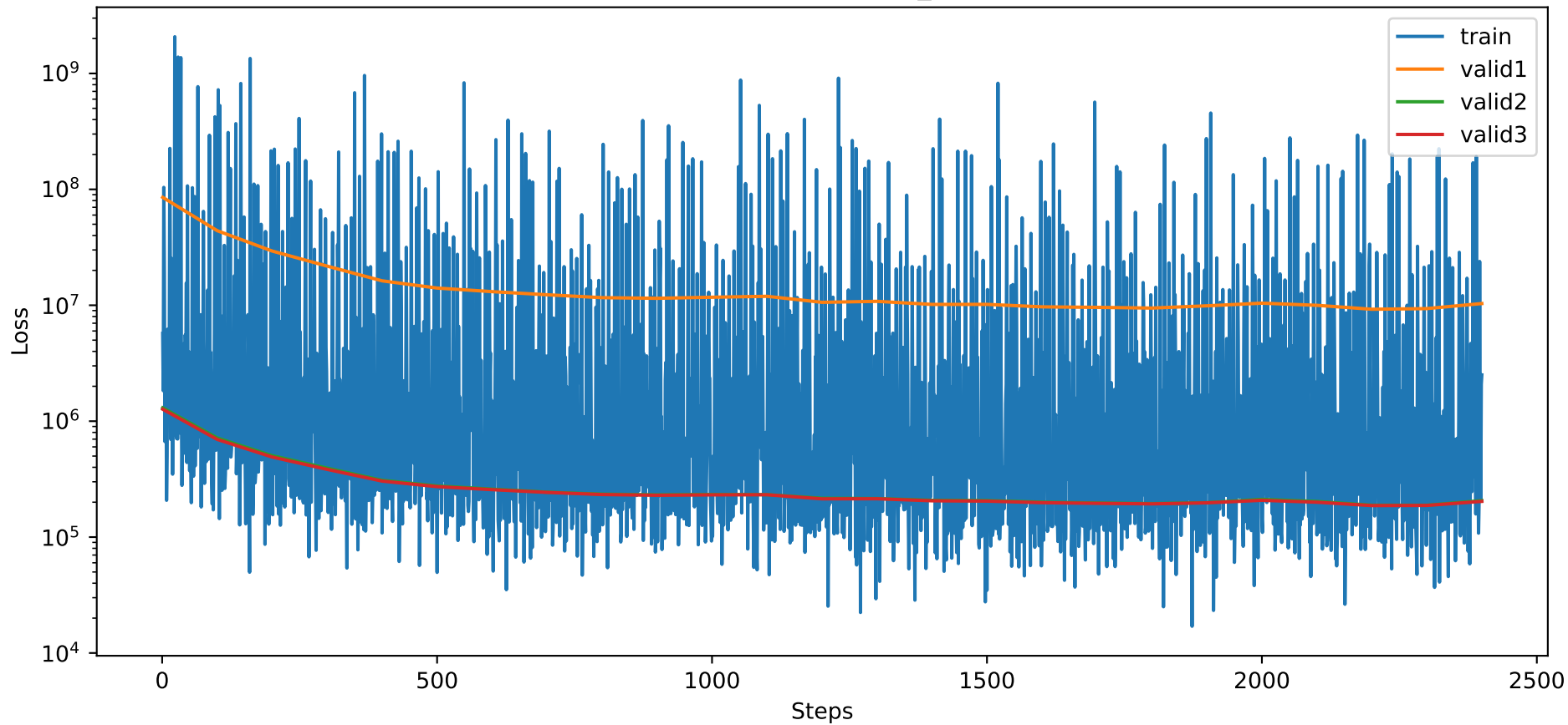
Training MSE of DLinear_instance
