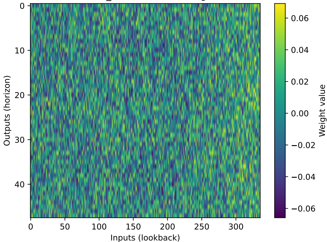
DLinear_instance trend weights
