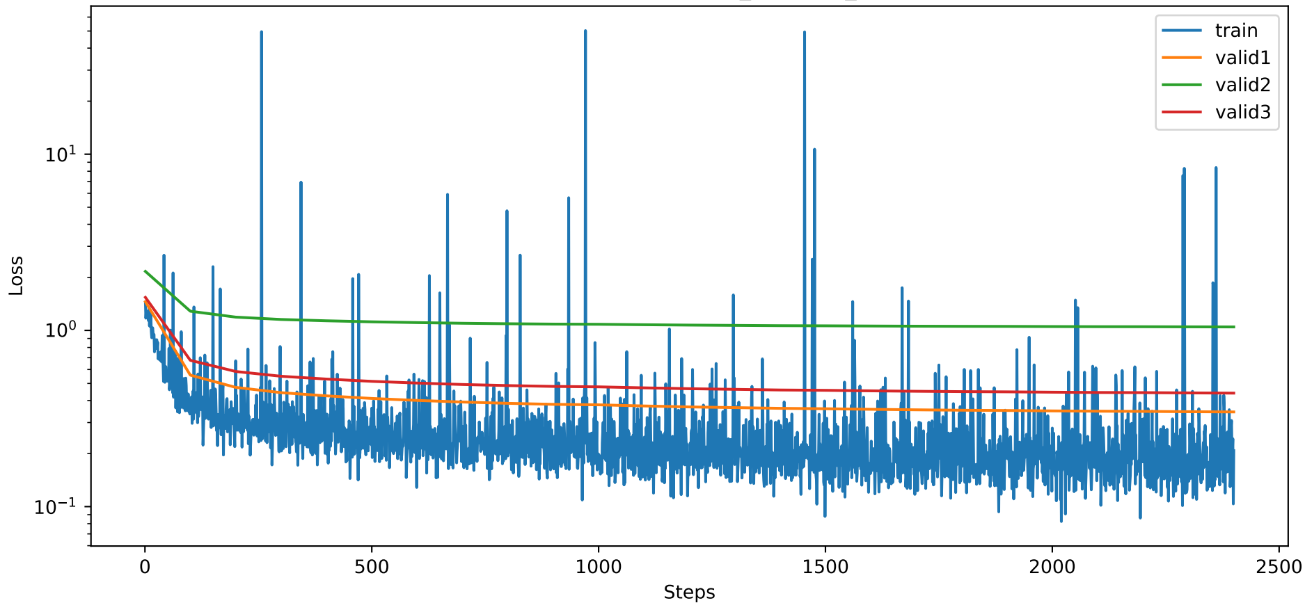
Training NMSE of DLinear_instance_NMSE
