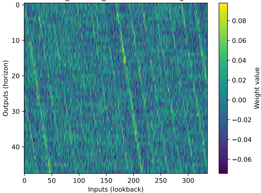
DLinear_instance_RMSE seasonal weights
