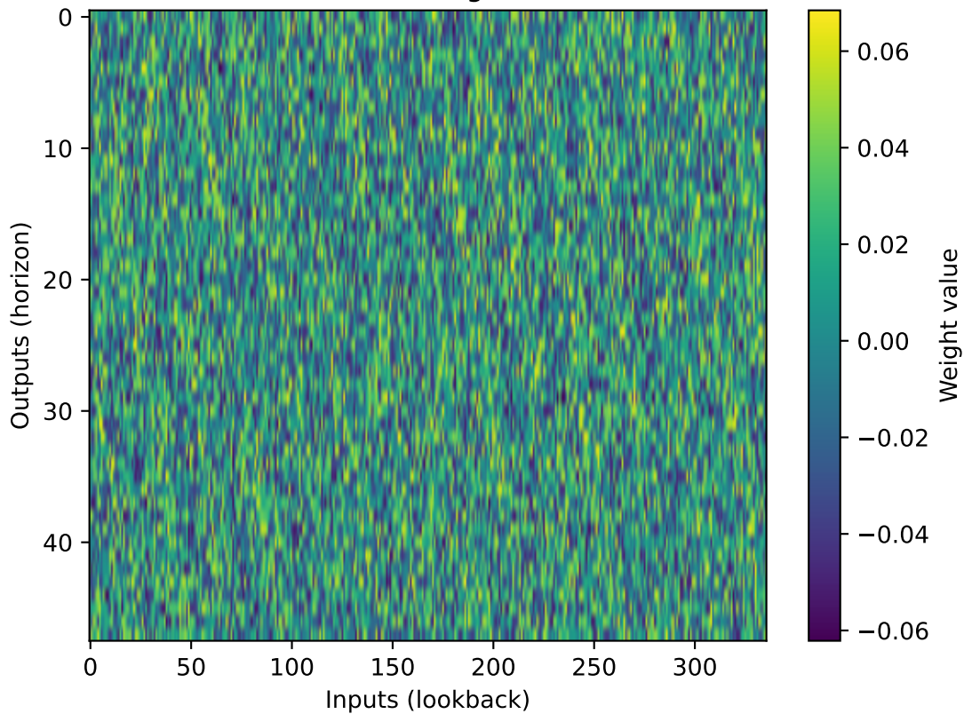
linear weights
