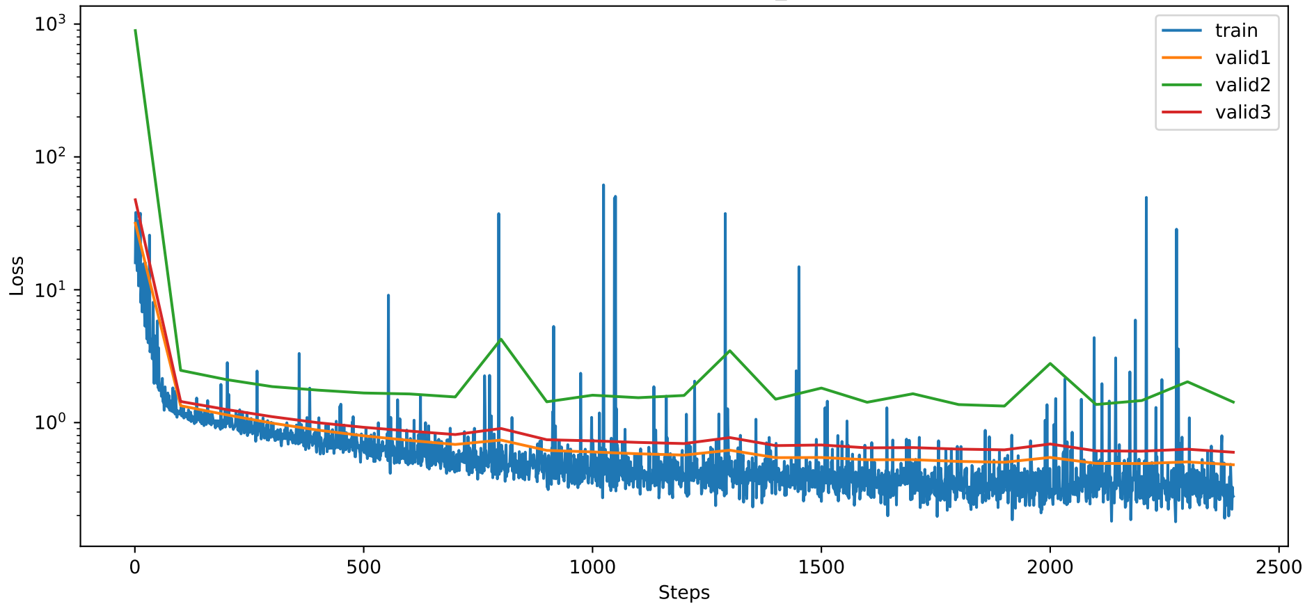
Training NMSE of linear_NMSE
