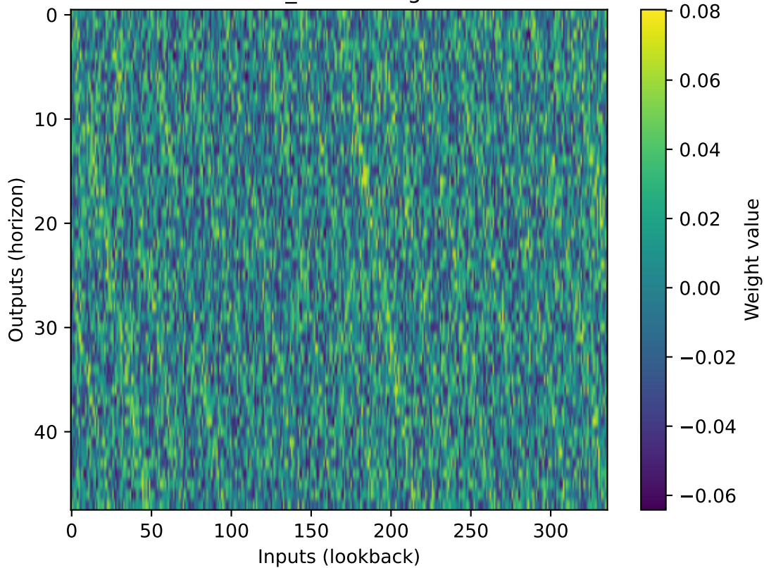
linear_NMSE weights
