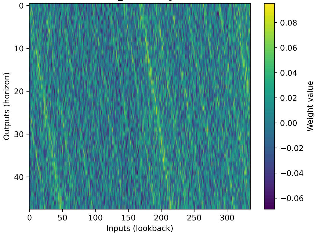
linear_RMSE weights
