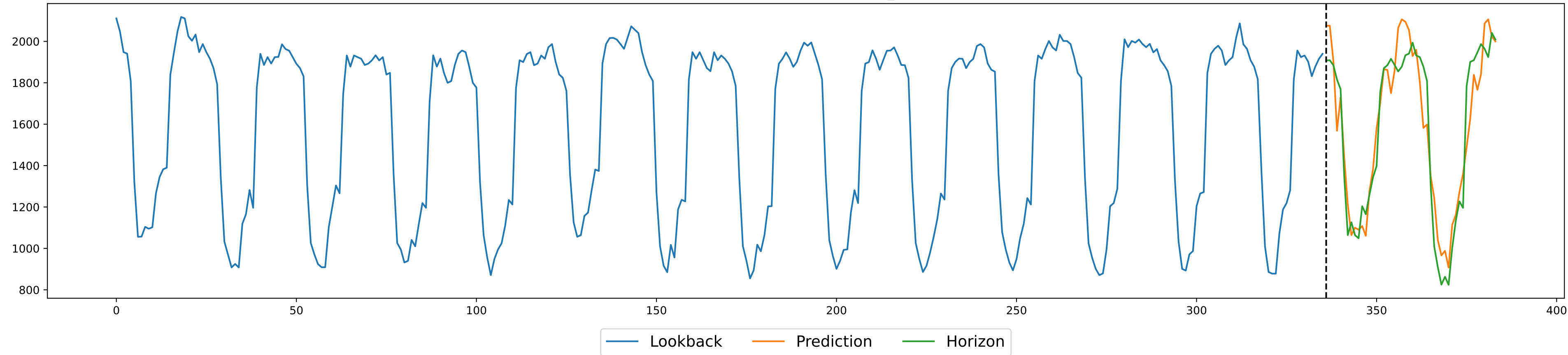
Example rand prediction for linear_instance
