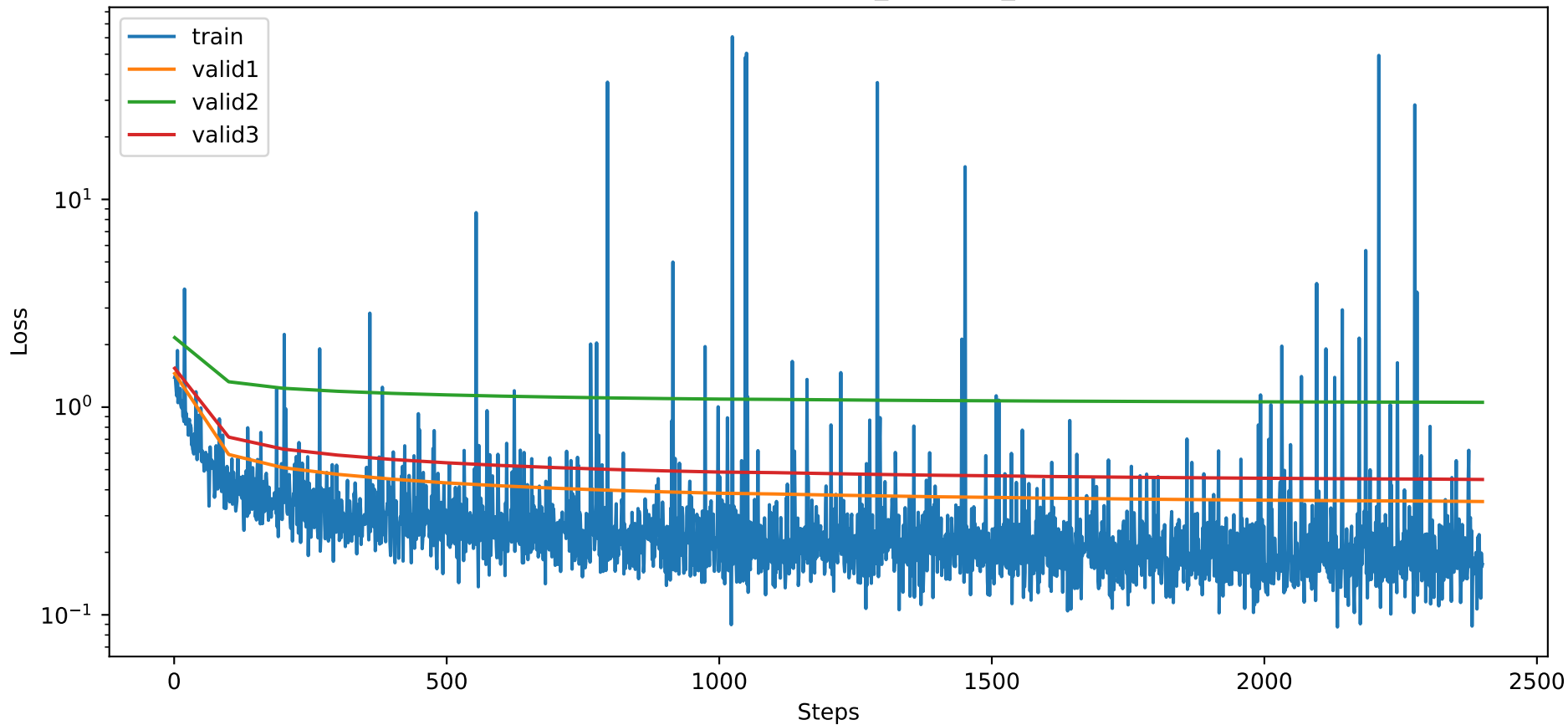
Training NMSE of linear_instance_NMSE
