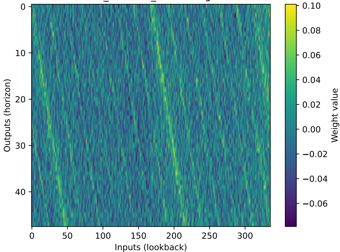
linear_instance_RMSE weights
