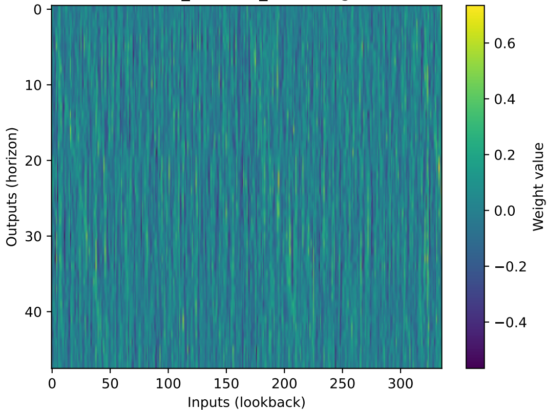
sklinear_instance_indiv weights
