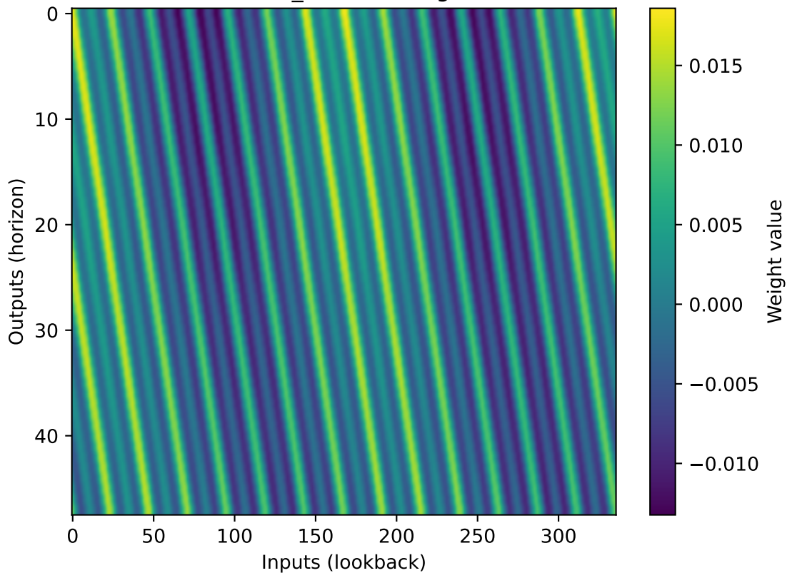
sklinear_relative weights
