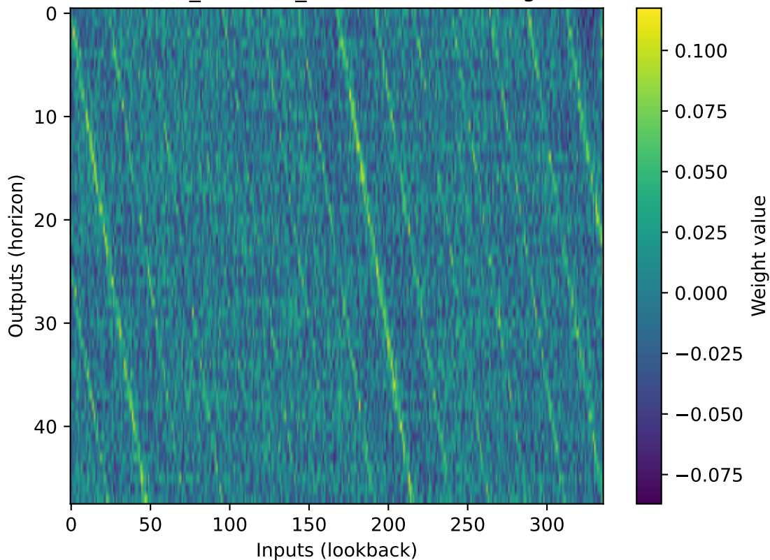
DLinear_instance_NMSE seasonal weights
