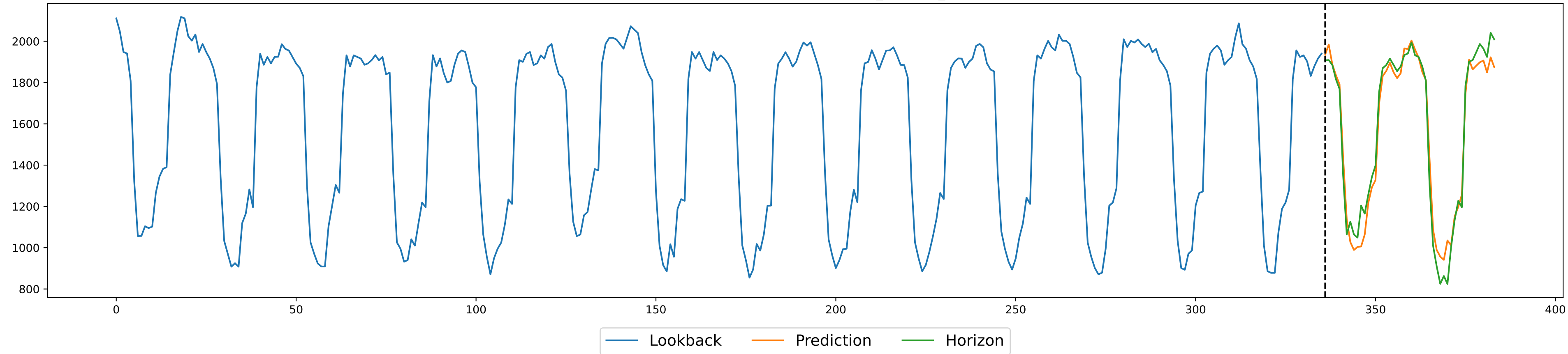
Example rand prediction for PatchTST_instance_NMSE
