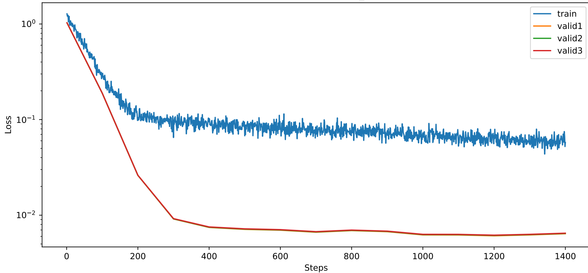
Training NMSE of min_init
