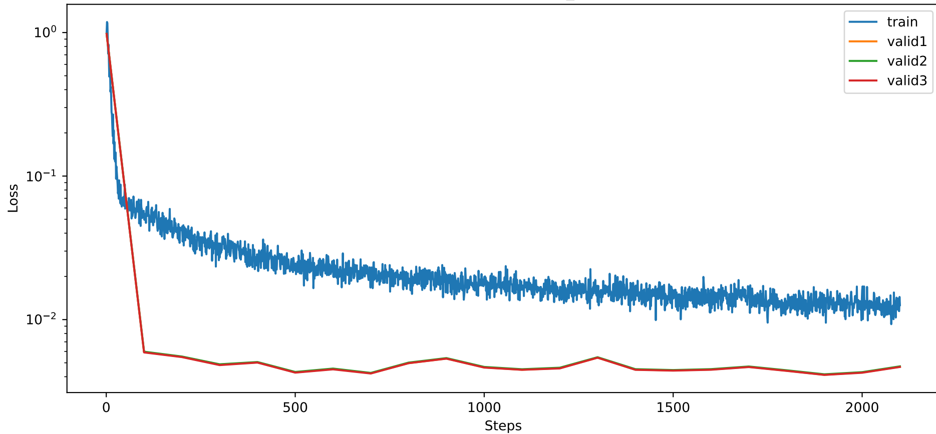
Training MSE of PatchTST_instance
