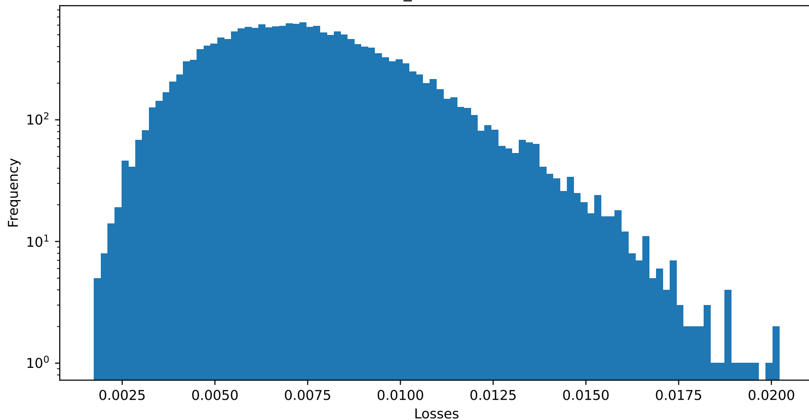
Test 1 NMSE of PatchTST_revin : 0.007577524520456791
