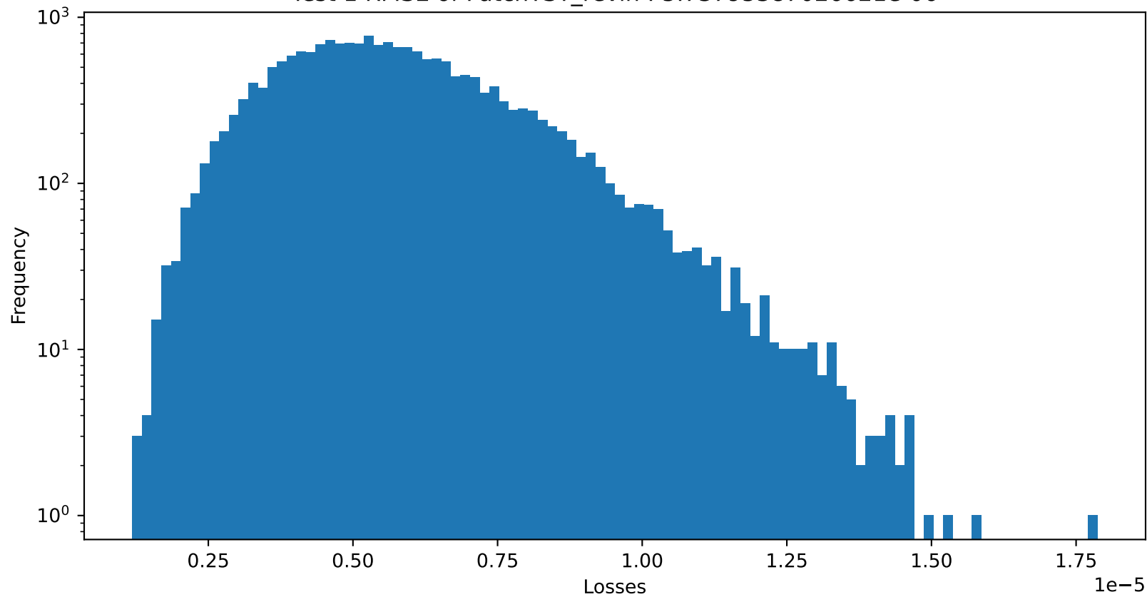
Test 1 RMSE of PatchTST_revin : 5.73795387026621e-06
