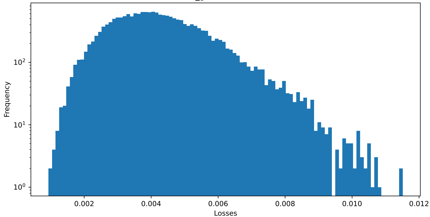
Test 1 MSE of default_gamma : 0.004282037727534771
