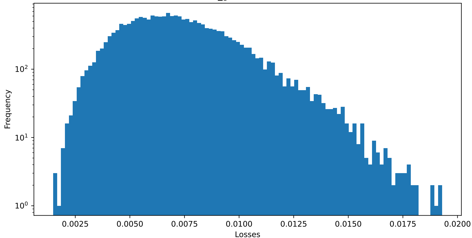
Test 1 NMSE of default_gamma : 0.007252320647239685
