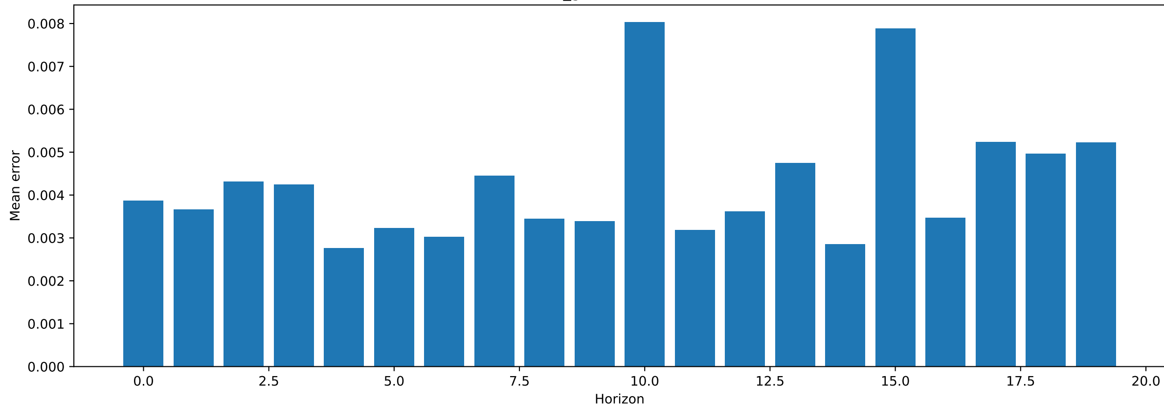
Test 1 MSE of default_gamma : 0.004282037727534771
