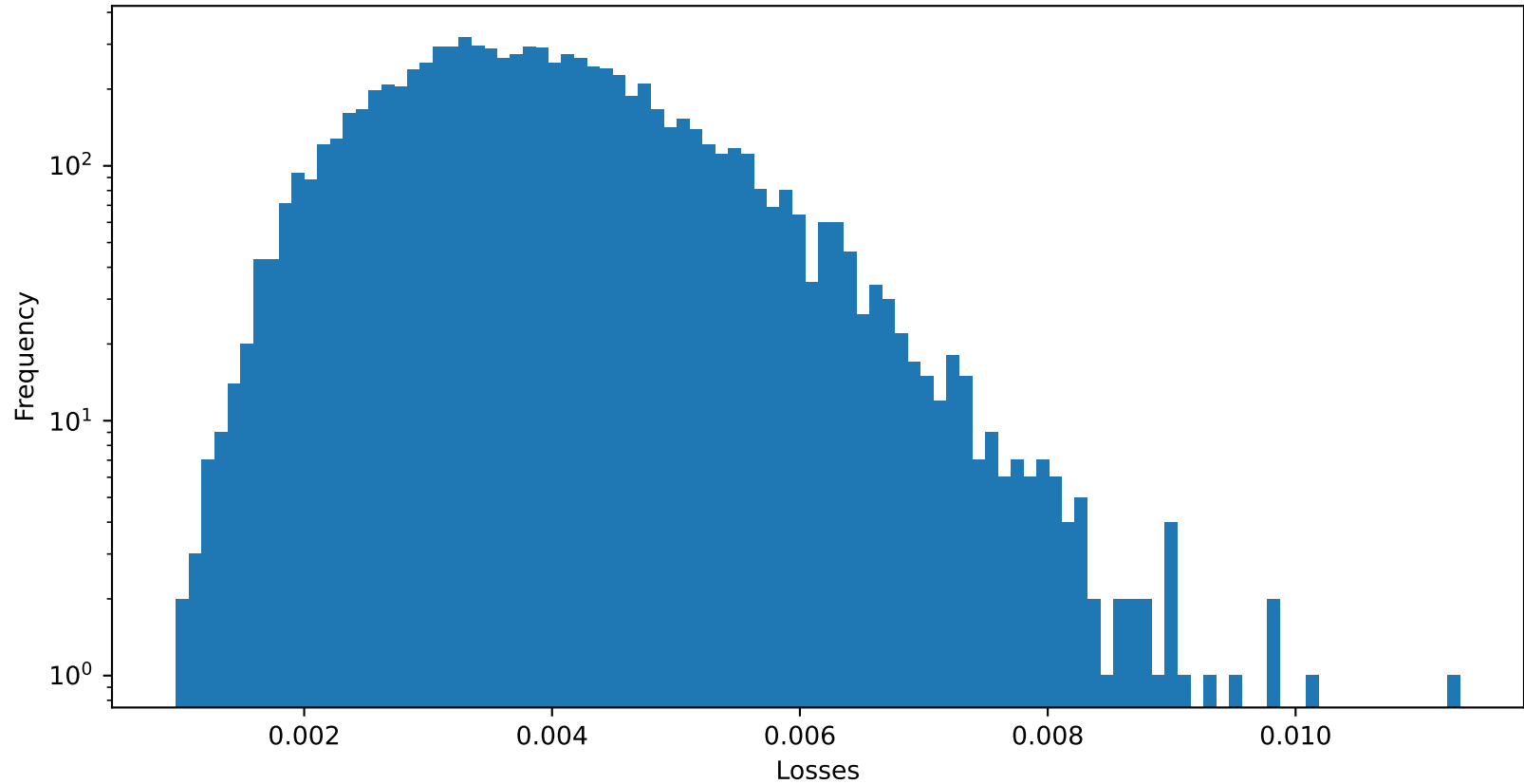
Test 2 MSE of fixed : 0.003921983297914267
