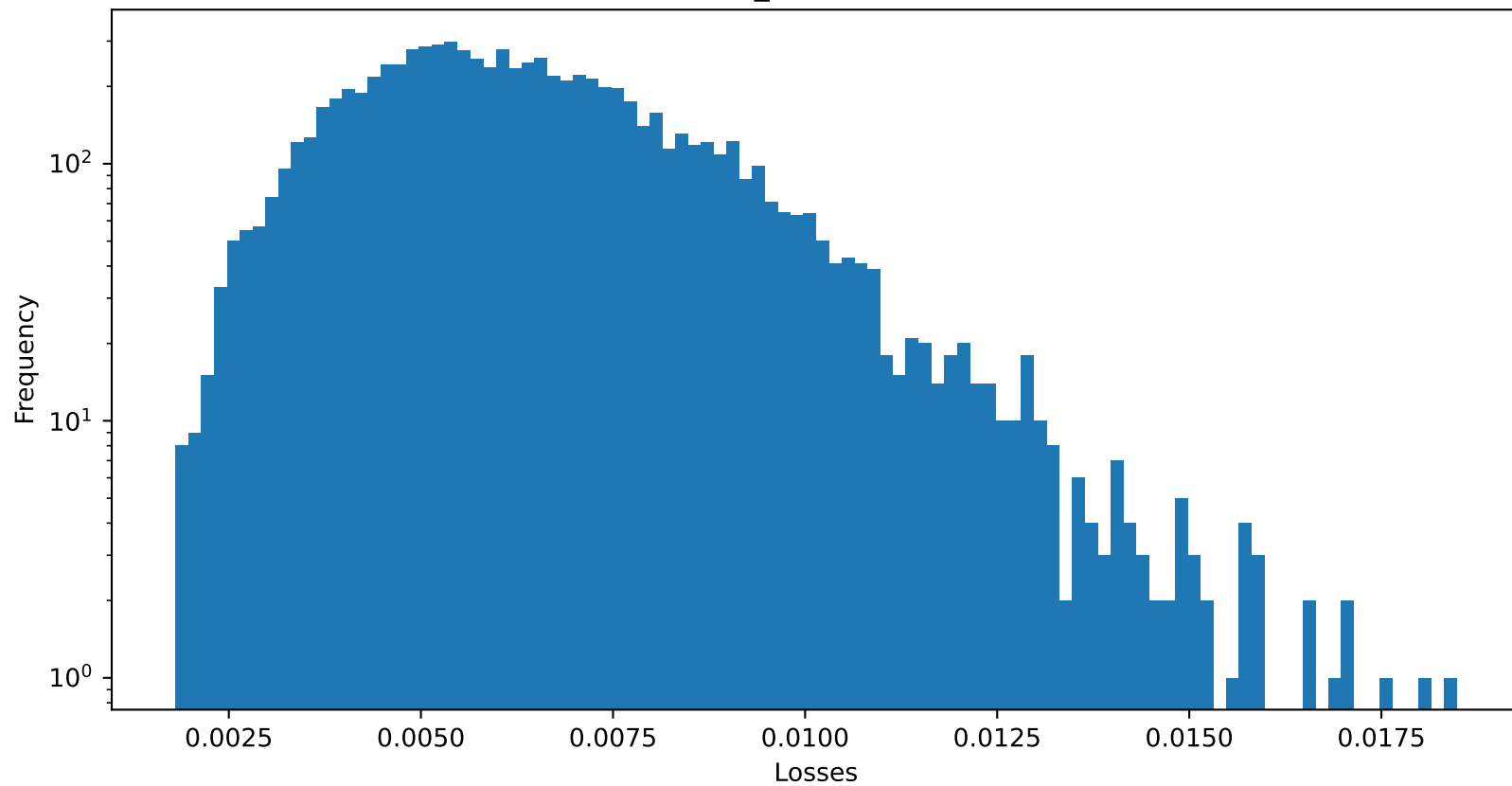
Test 2 NMSE of PatchTST_revin : 0.006396139971911907
