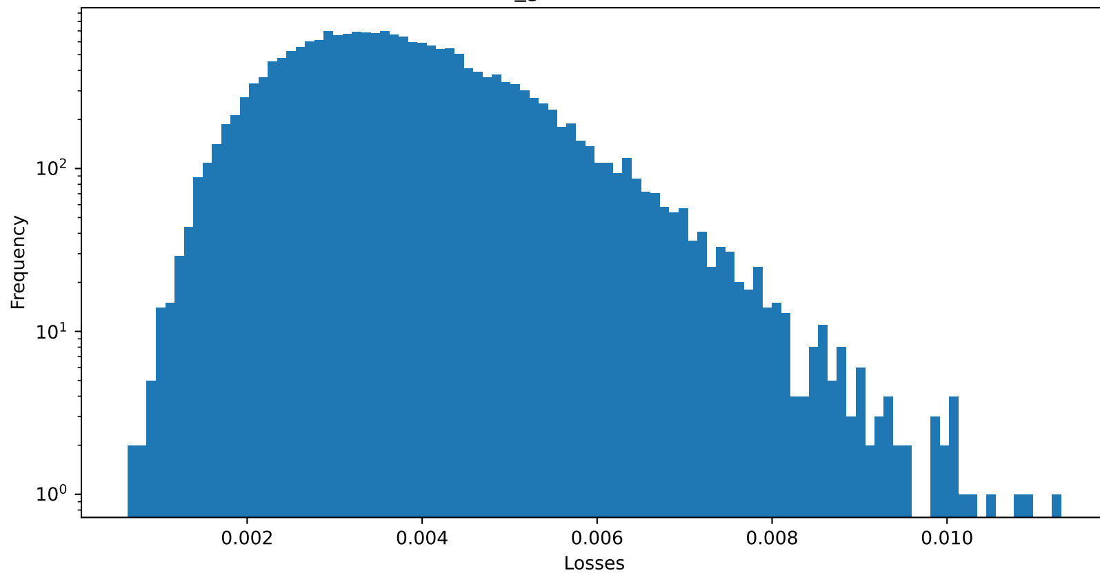
Test 1 MSE of default_gamma : 0.003781089326366782
