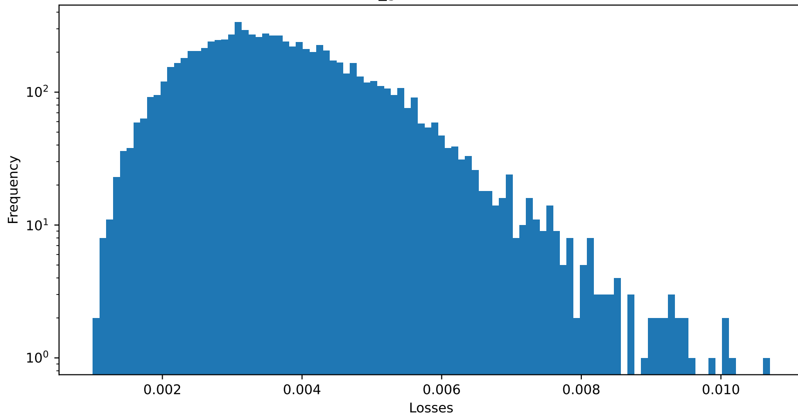
Test 2 MSE of default_gamma : 0.00372925098054111
