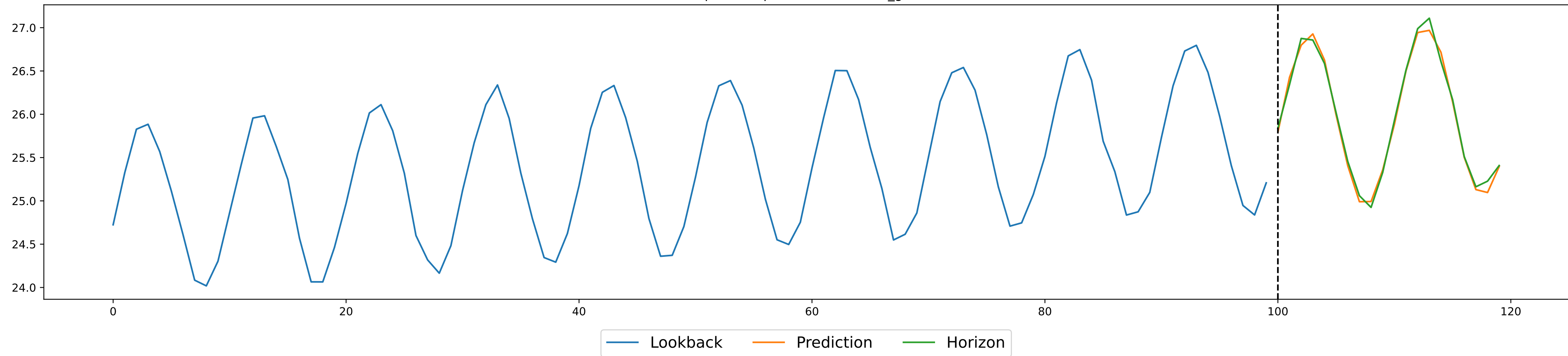
Example rand prediction for fixed_gamma
