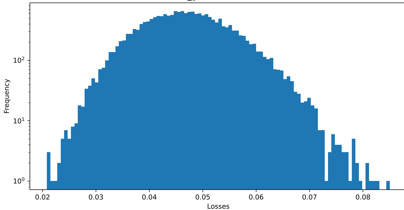
Test 1 MAE of fixed_gamma : 0.04709892347455025
