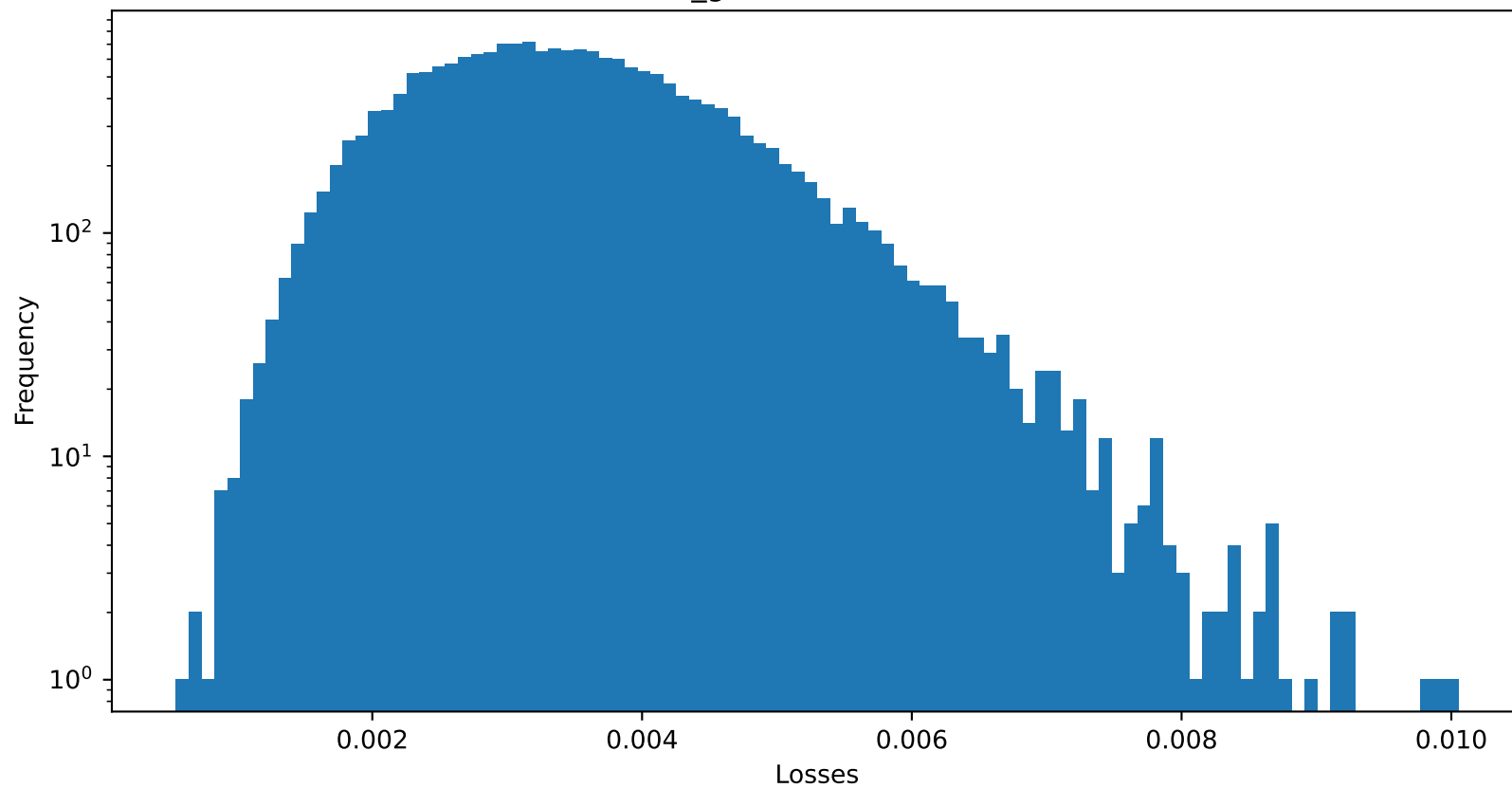
Test 1 MSE of fixed_gamma : 0.003500328864902258
