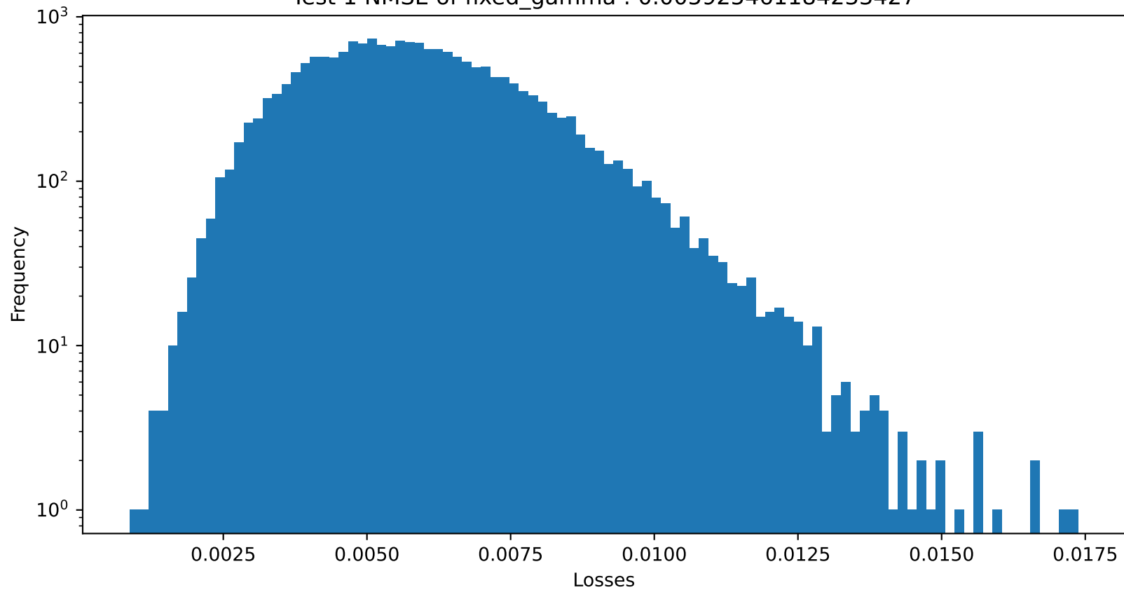
Test 1 NMSE of fixed_gamma : 0.005925461184233427
