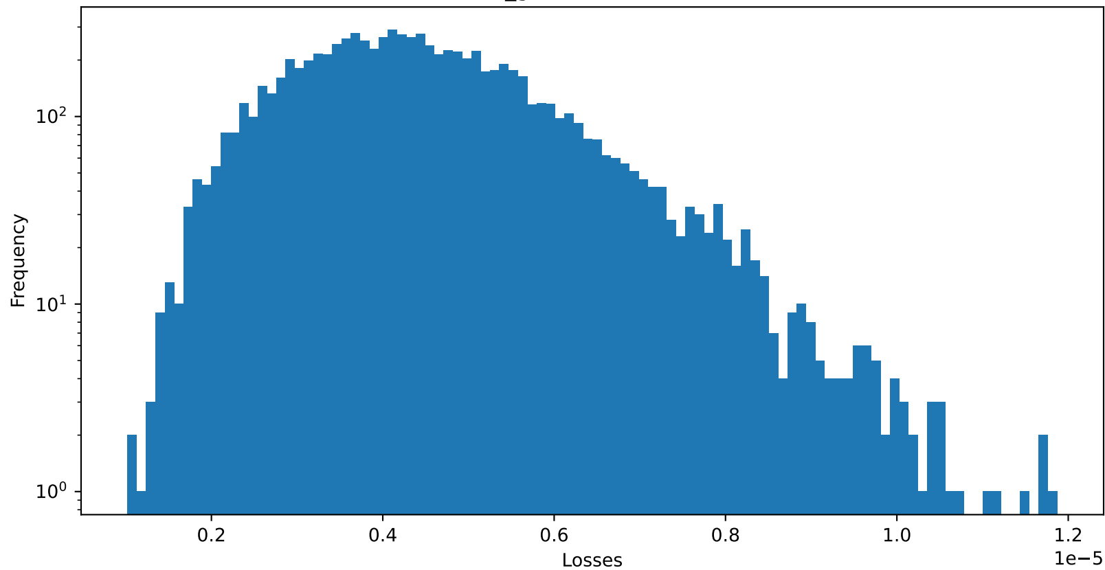
Test 2 RMSE of fixed_gamma : 4.469383384275716e-06
