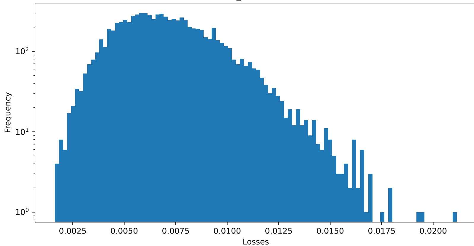
Test 2 NMSE of PatchTST_revin : 0.007164363283663988
