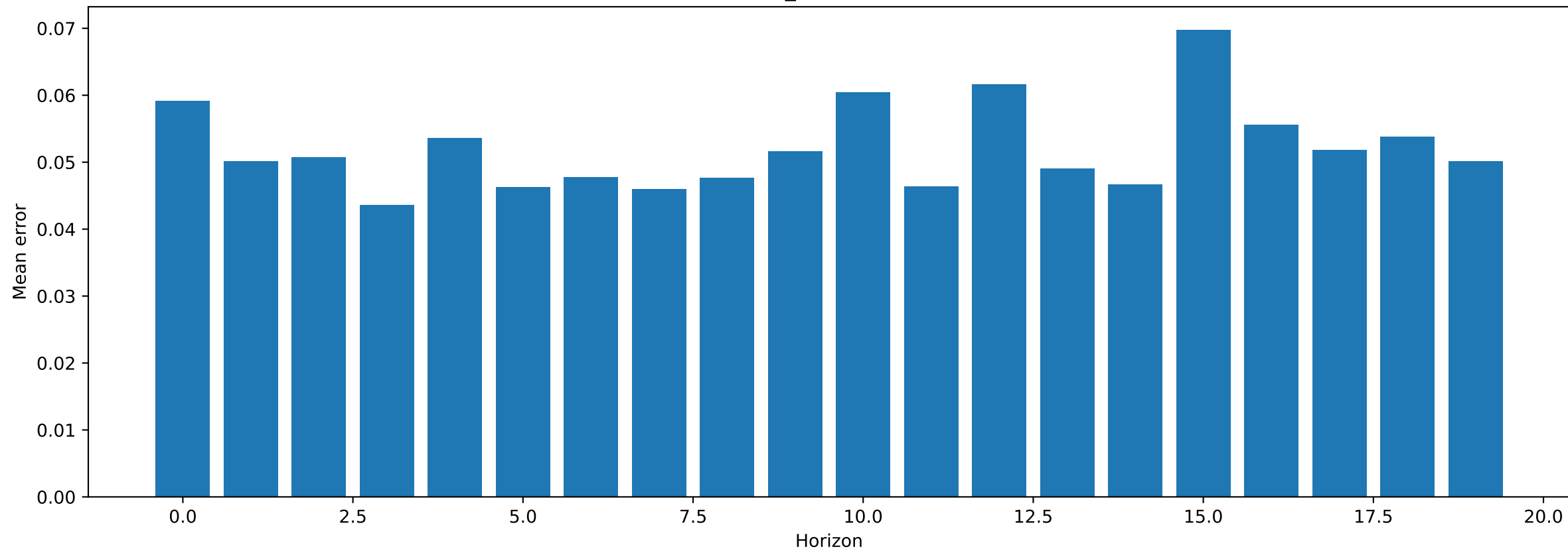
Test 2 MAE of PatchTST_revin : 0.05209923908114433
