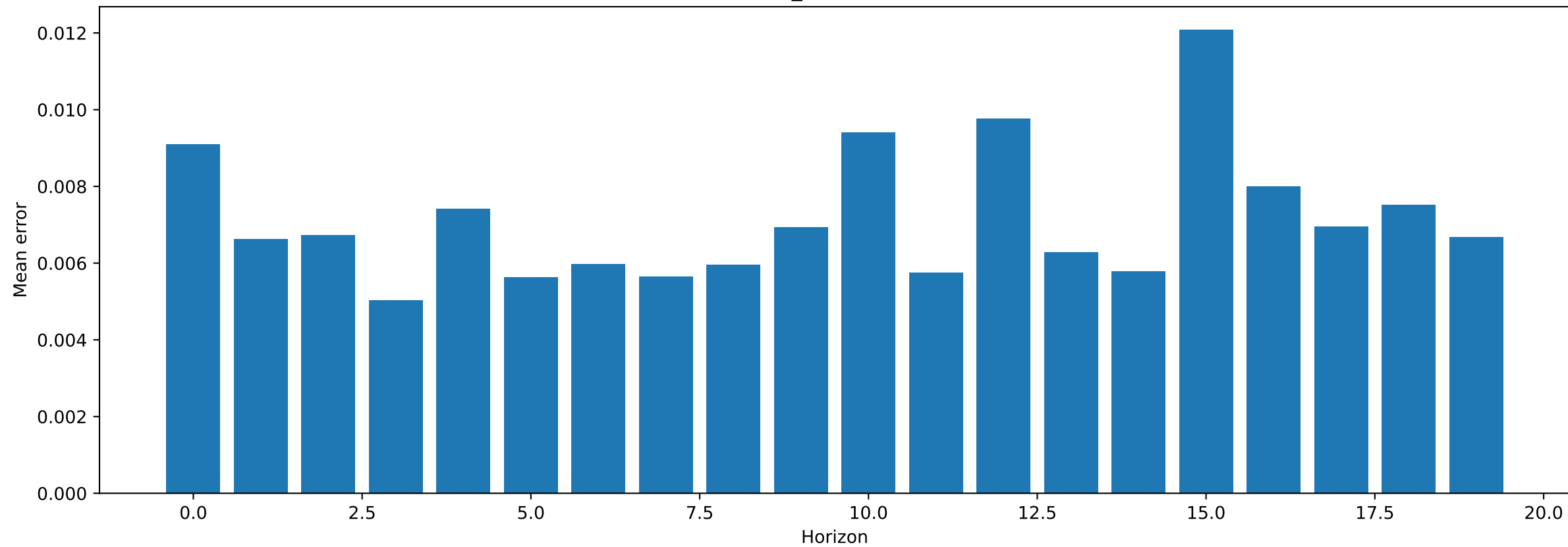
Test 2 NMSE of PatchTST_revin : 0.007164363283663988
