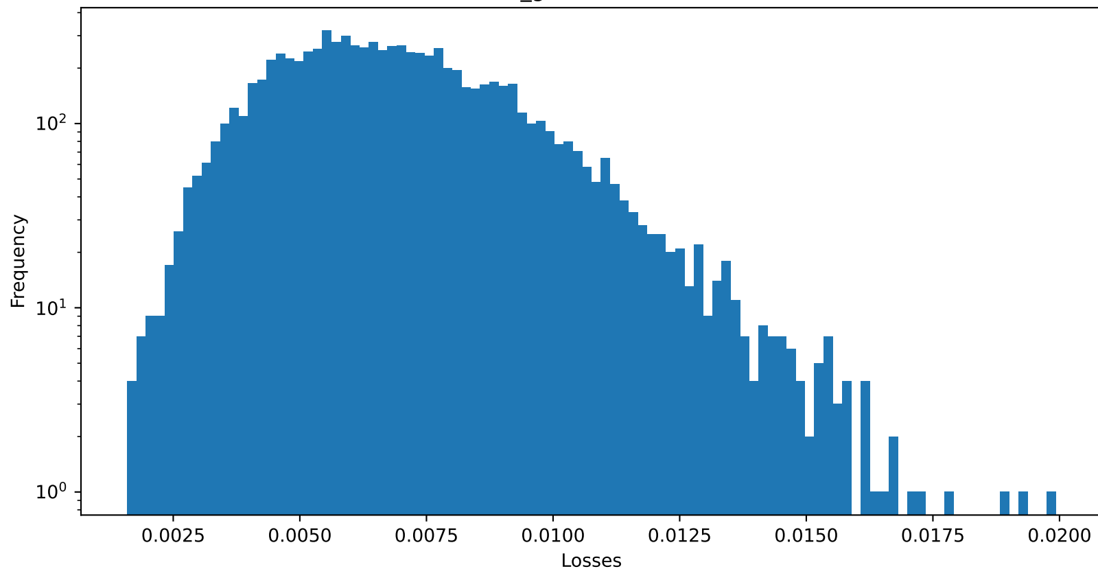
Test 2 NMSE of default_gamma : 0.006904588080942631
