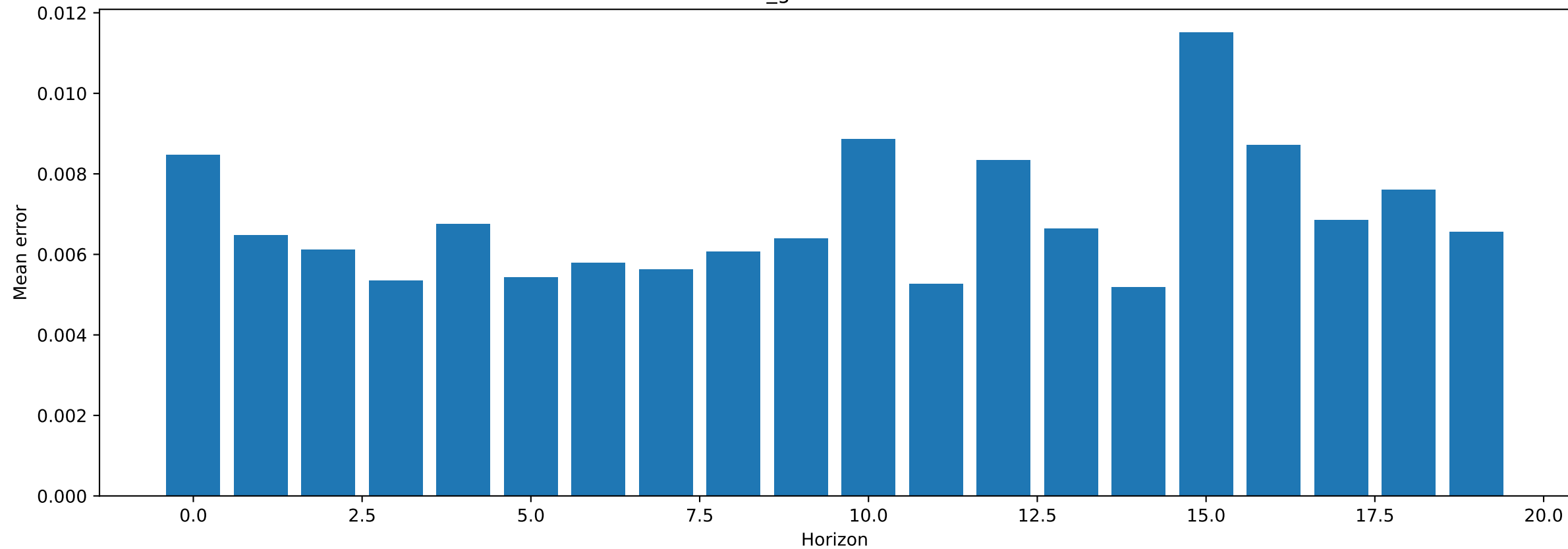
Test 2 NMSE of default_gamma : 0.006904588080942631
