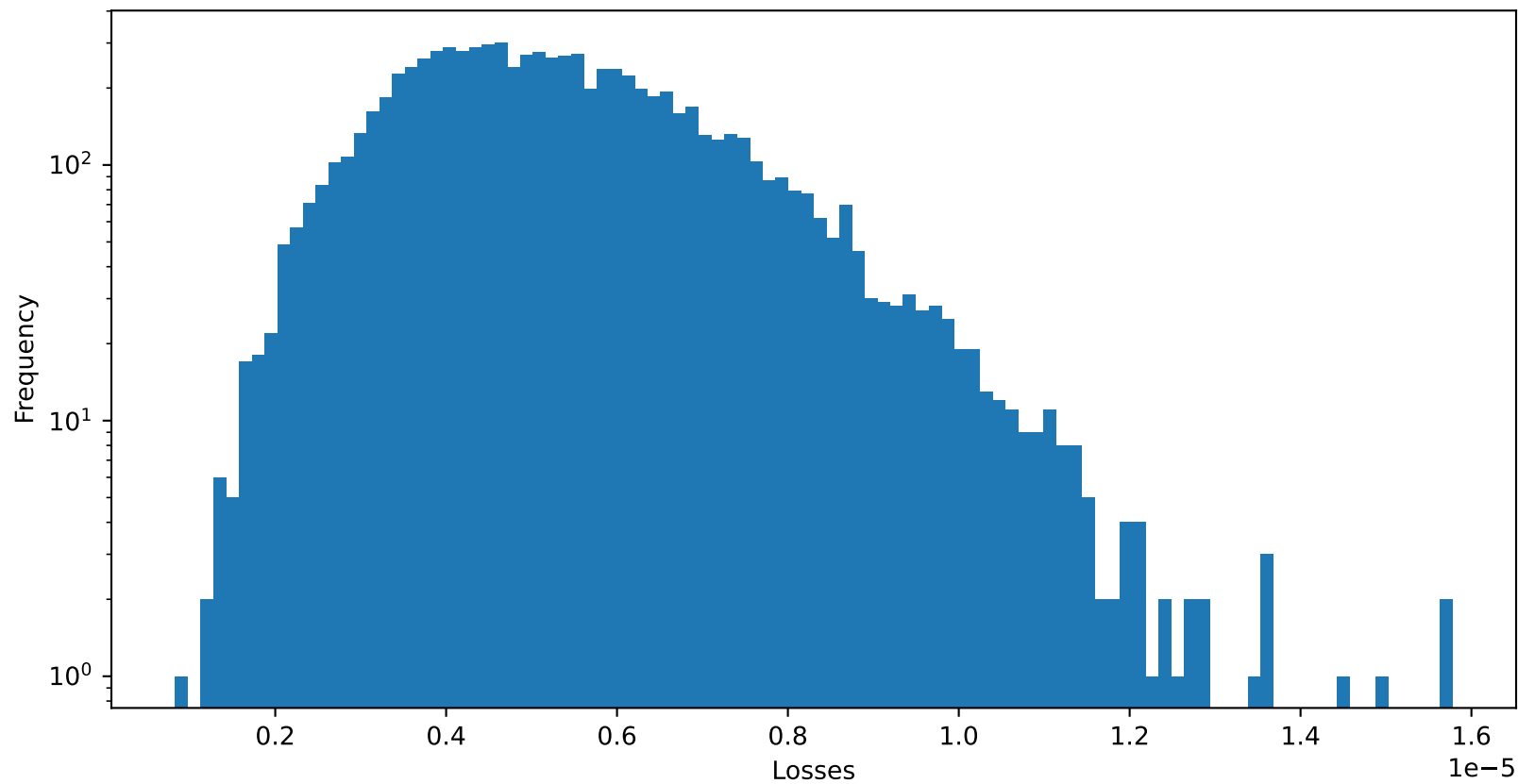
Test 2 RMSE of fixed : 5.358918315323535e-06
