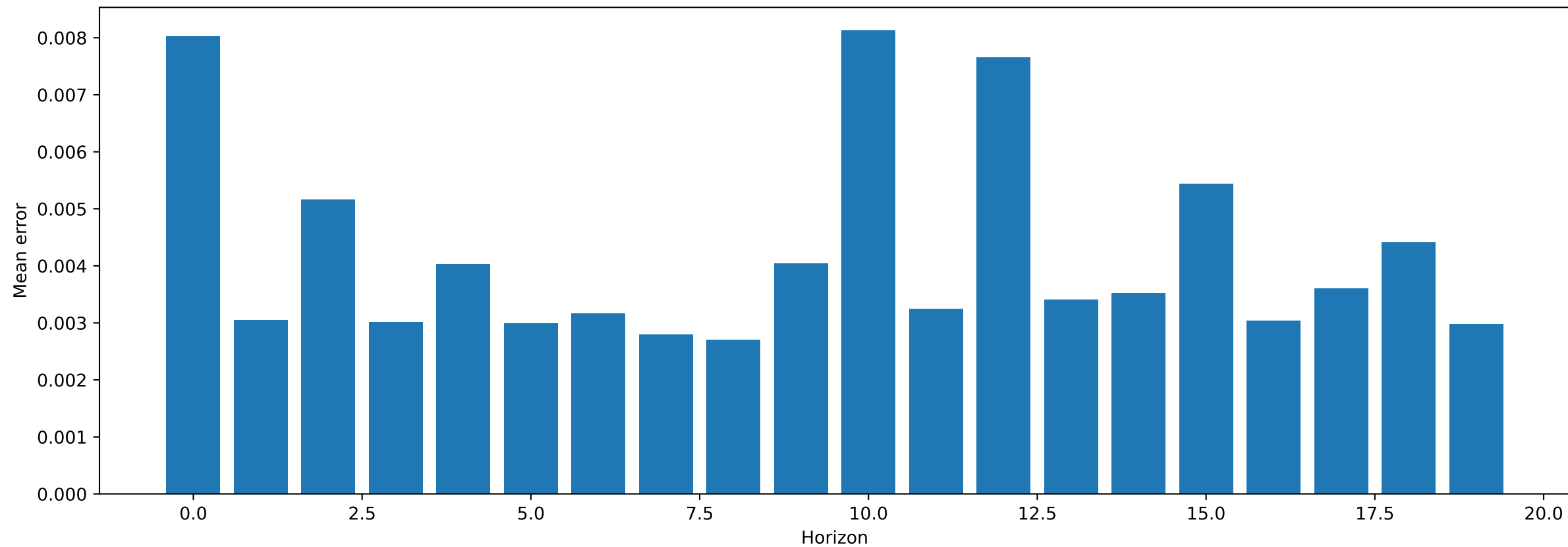
Test 2 MSE of fixed : 0.004222920164465904
