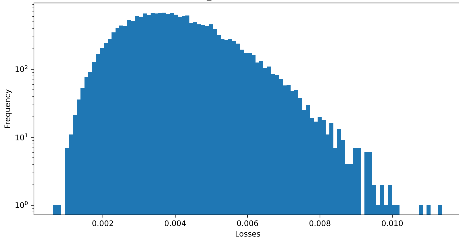
Test 1 MSE of fixed_gamma : 0.0040023839101195335
