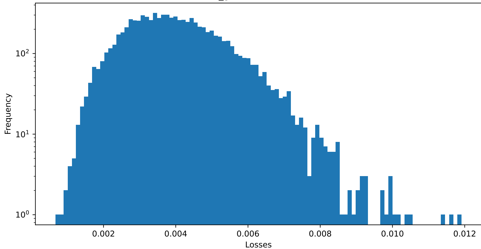
Test 2 MSE of fixed_gamma : 0.004021402448415756
