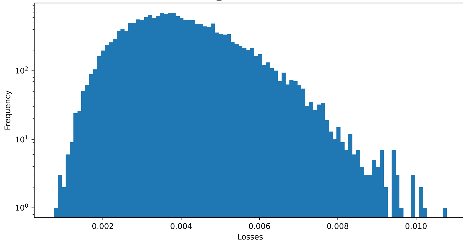
Test 1 MSE of default_gamma : 0.003977177664637566
